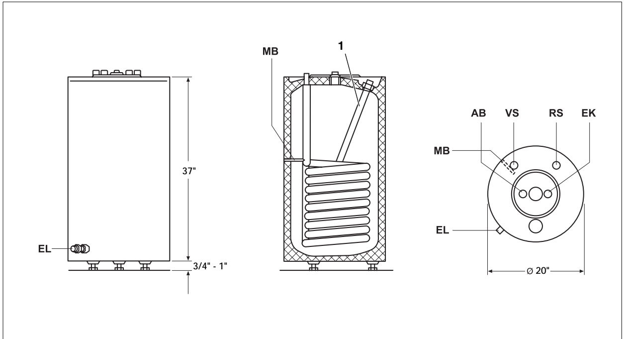
Fig. 4 Dimensions and piping connections (measurements in inches)
