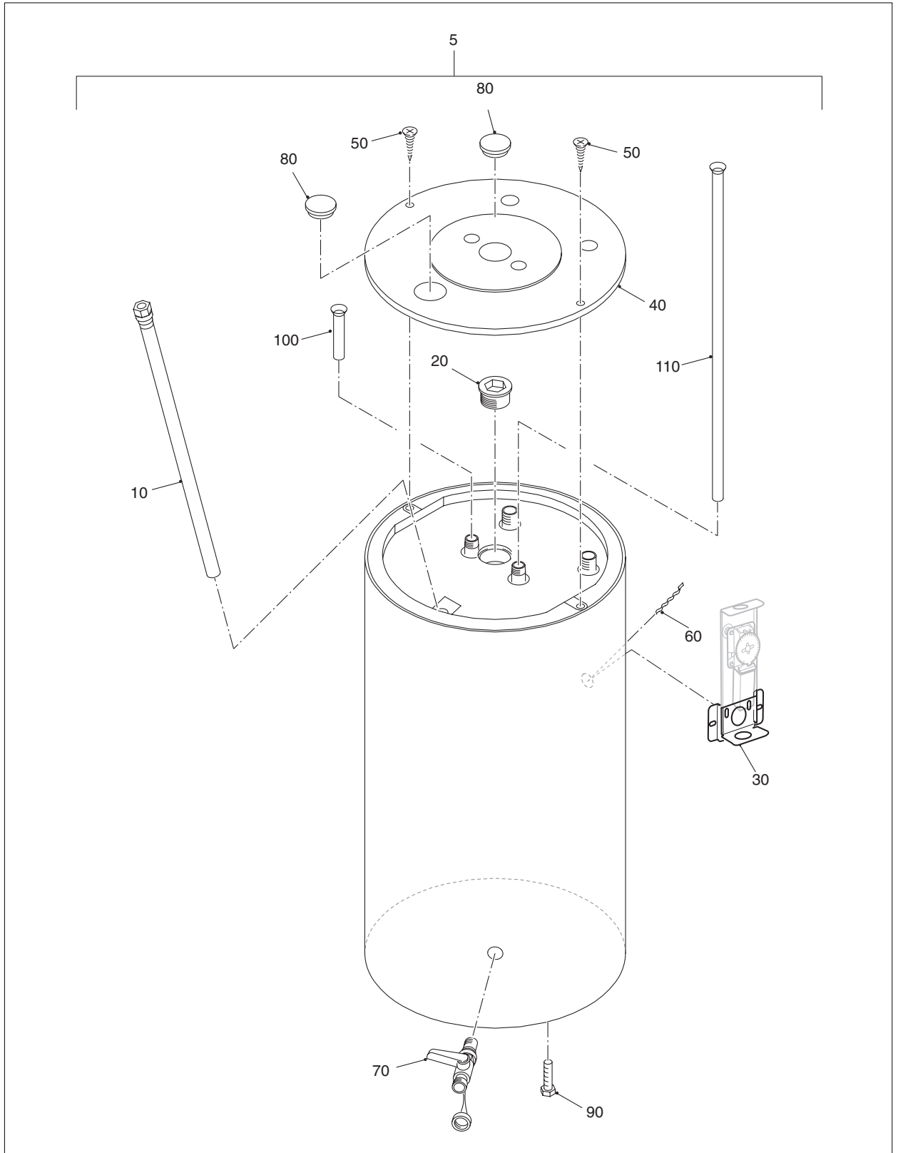
Fig. 12 Spare Parts for S120
