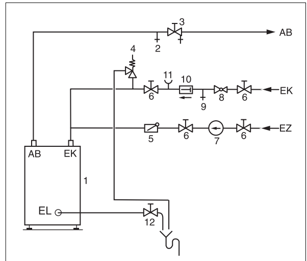
Fig. 6 Tank piping installation (sample picture)
