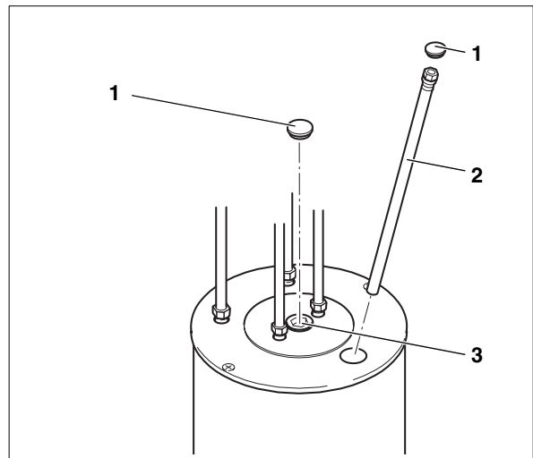
Fig. 10 Removal of magnesium anode rod
