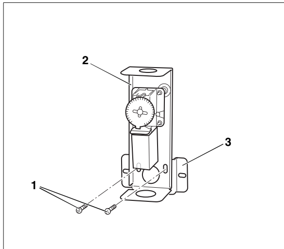
Fig. 8 Attaching bracket to aquastat
