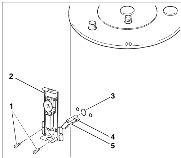
Fig. 9 Installation of Honeywell aquastat
