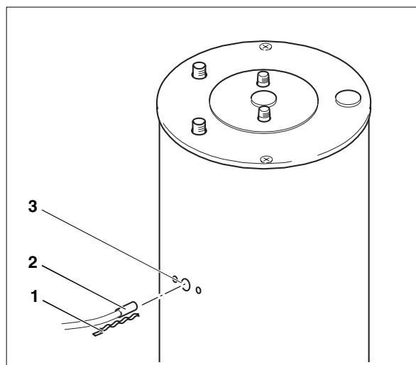
Fig. 7 Installation of temperature sensor
