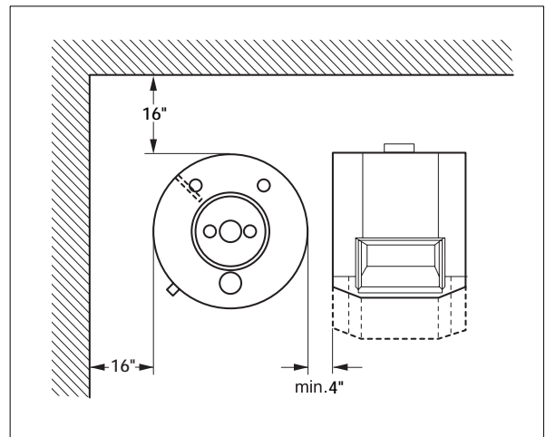
Fig. 1 Recommended clearance for installation and maintenance.
